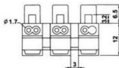
PA11-3 3 poles
