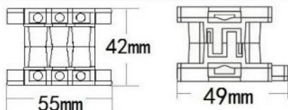
M29-W02 (Small) NO. : 2P/3P
