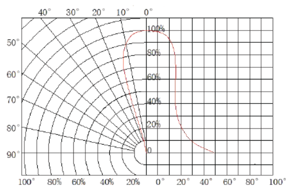
Radiation diagram
