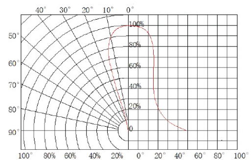
Radiation diagram
