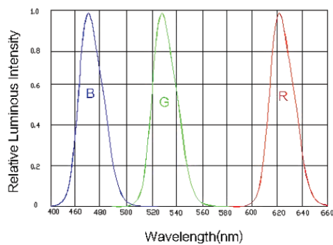
Relative Spectral emission
