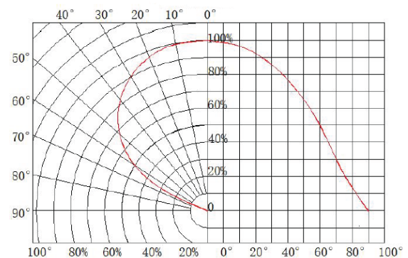
Radiation diagram
