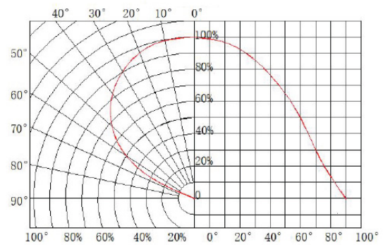
Radiation diagram
