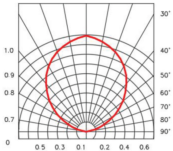
Radiation diagram 0° 10° 20°
