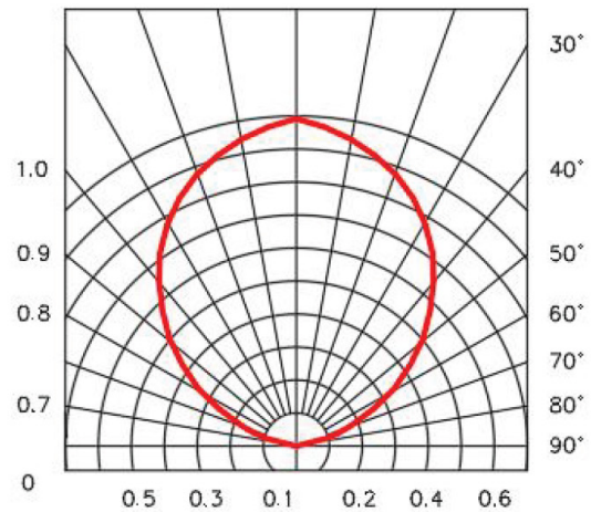
Radiation diagram 0° 10° 20°
