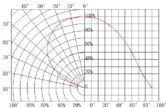
Radiation diagram
