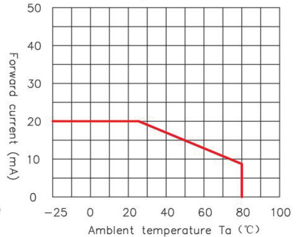
Forward current derating curve Vs. Ambient temperature
