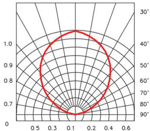
Radiation diagram 0° 10° 20°
