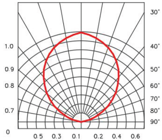
Radiation diagram 0° 10° 20°
