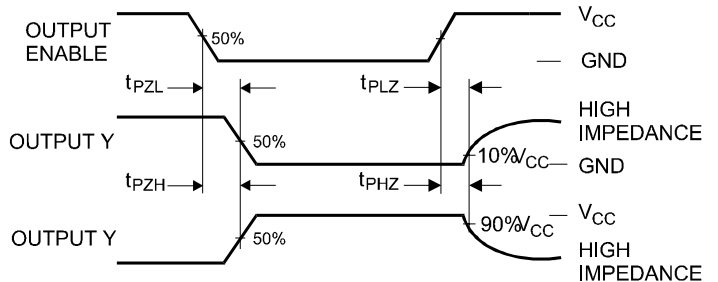
Figure 2. Switching Waveforms
