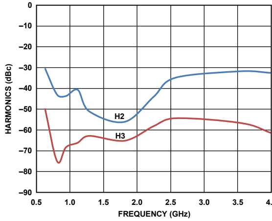
Figure 25. Single-Tone Harmonics vs. Frequency, P_{out} = 0 dBm
