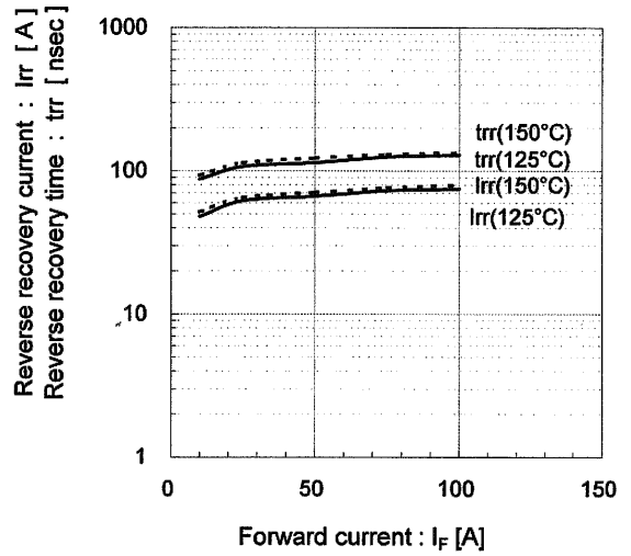
Reverse recovery characteristics (typ.) Vcc=600V, VGE=±15V, Rg=15Ω
