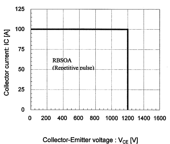
[ Inverter ] Reverse bias safe operating area (max.) +V_{GE}=15V, -V_{GE} \le 15V, R_g \ge 15\Omega, T_j \le 125^\circ C
