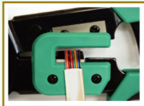
Cutting
