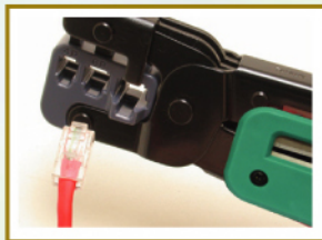
Crimping 4P/6P/8P
