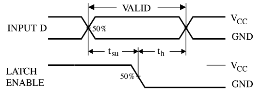
Figure 4. Switching Waveforms
