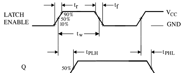
Figure 2. Switching Waveforms
