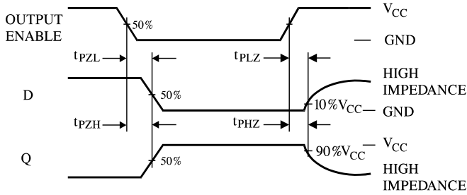
Figure 3. Switching Waveforms
