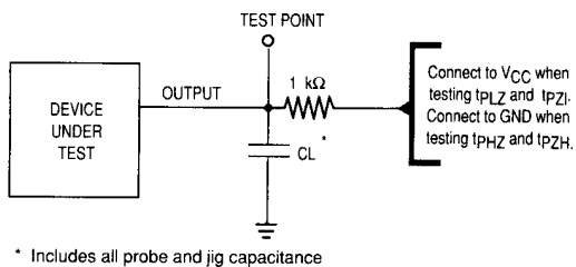
Figure 6. Test Circuit
