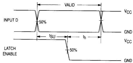
Figure 2. Switching Waveforms
