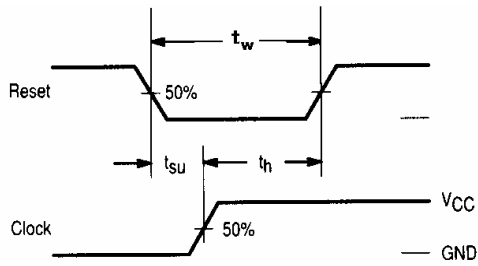
Figure 3. Switching Waveforms
